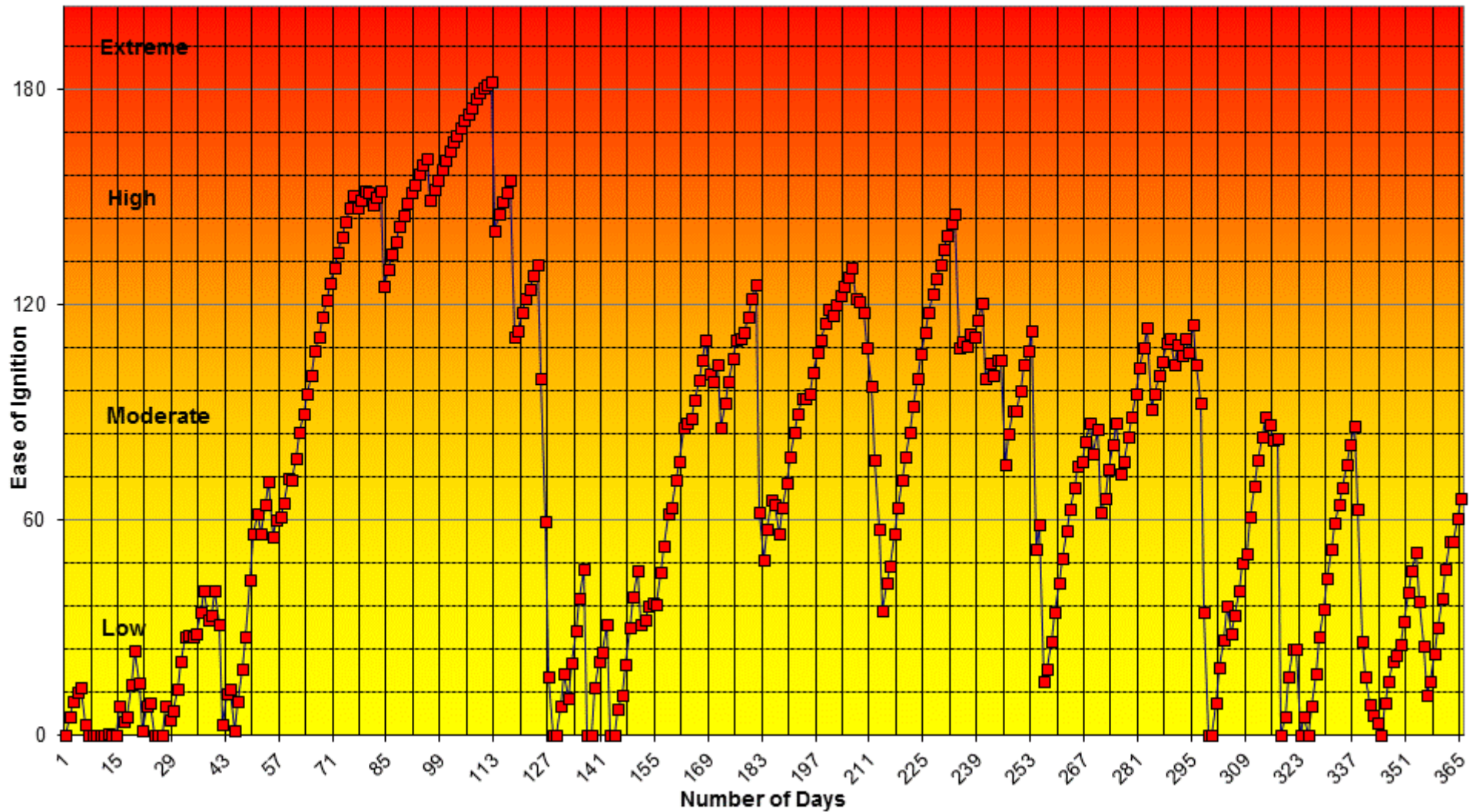
Keetch-Byram Dryness Index 2007
