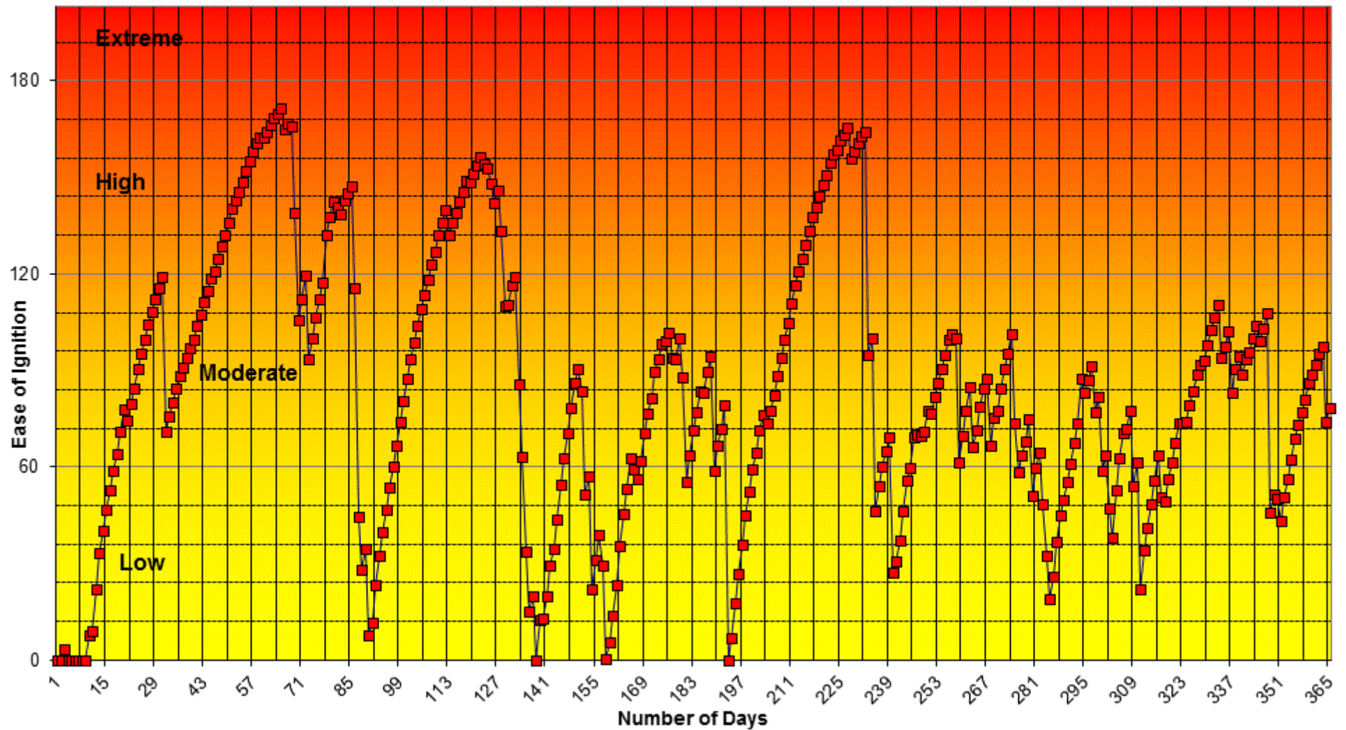
Keetch-Byram Dryness Index 2005
