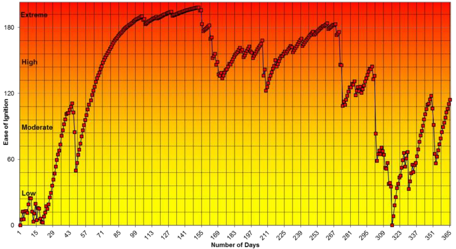
Keetch-Byram Dryness Index 2014
