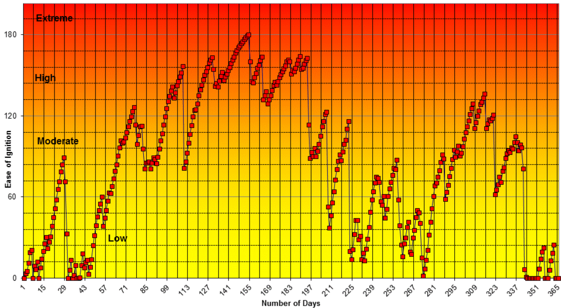
Keetch-Byram Dryness Index 2003
