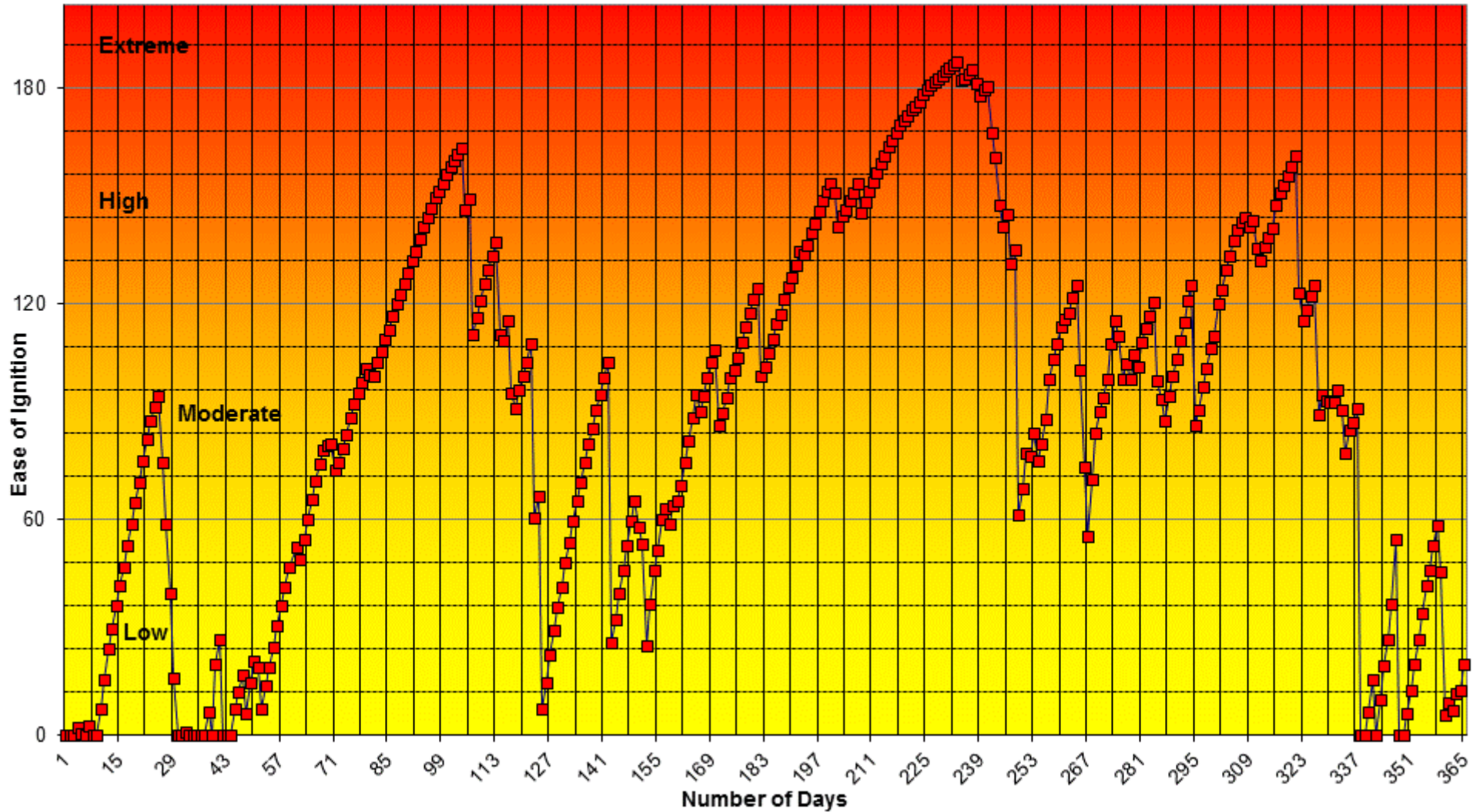
Keetch-Byram Dryness Index 2011
