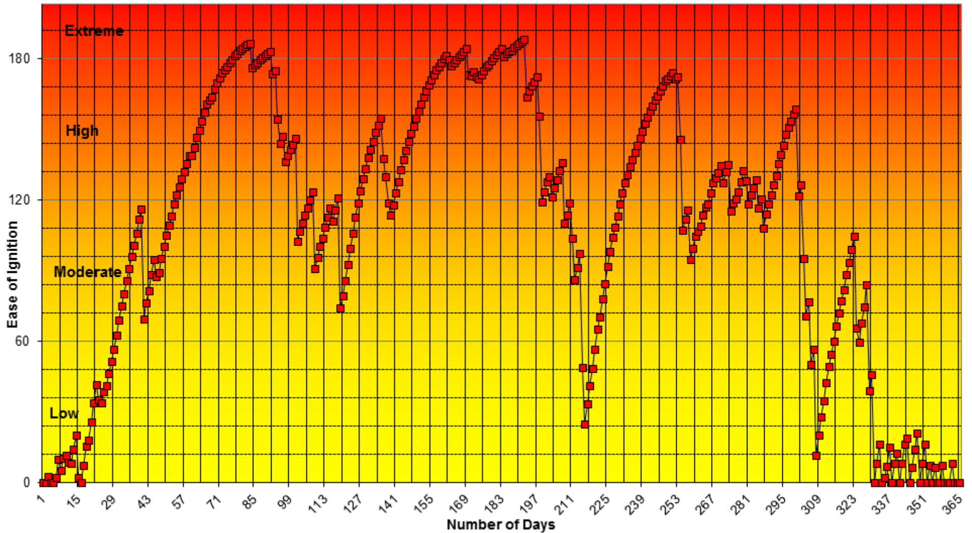
Keetch-Byram Dryness Index 2010
