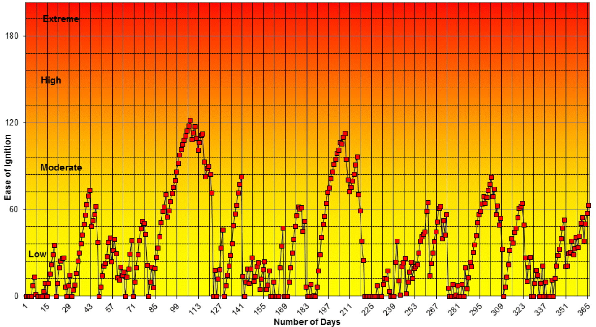
Keetch-Byram Dryness Index 2008
