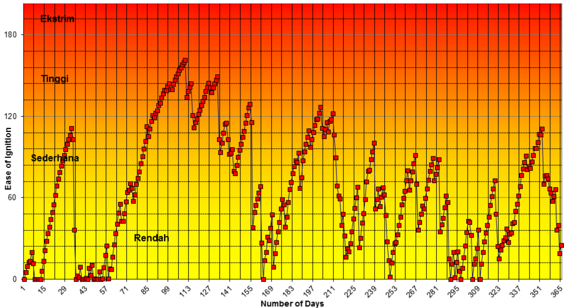
Keetch-Byram Dryness Index 2006
