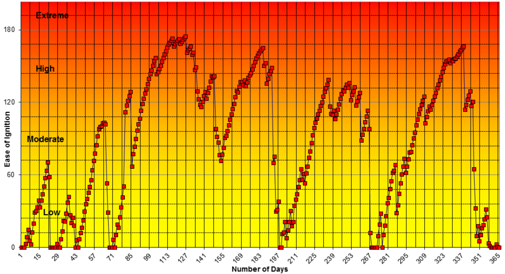
Keetch-Byram Dryness Index 2004
